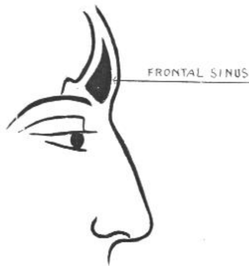
FRONTAL SINUS
